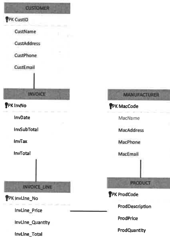
Figure 2.1 The partial entity relationship diagram (ERD) of product selling records
